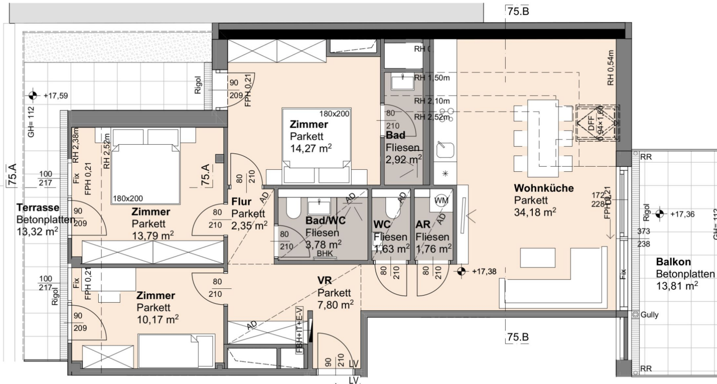
Top 1/75
