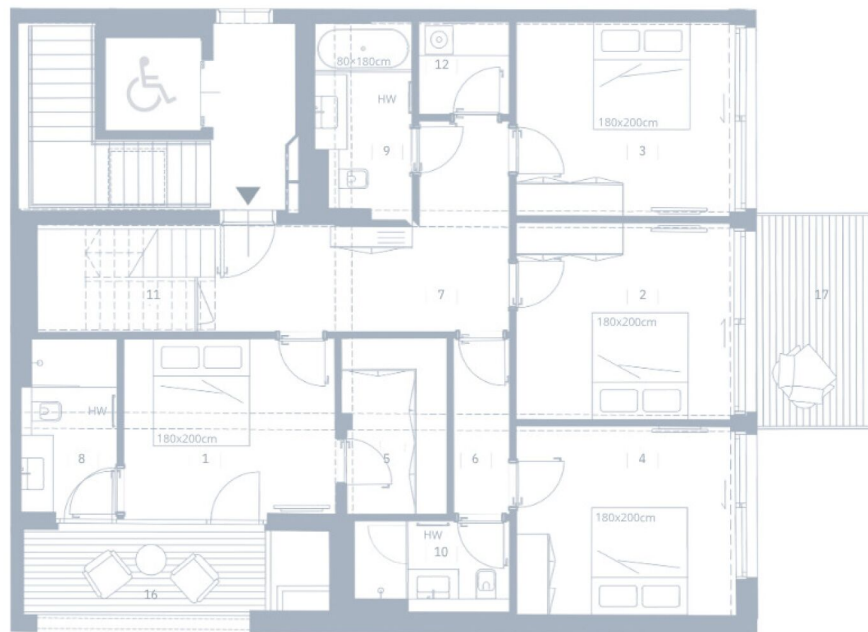
3. OBERGESCHOSS 3rd floor
