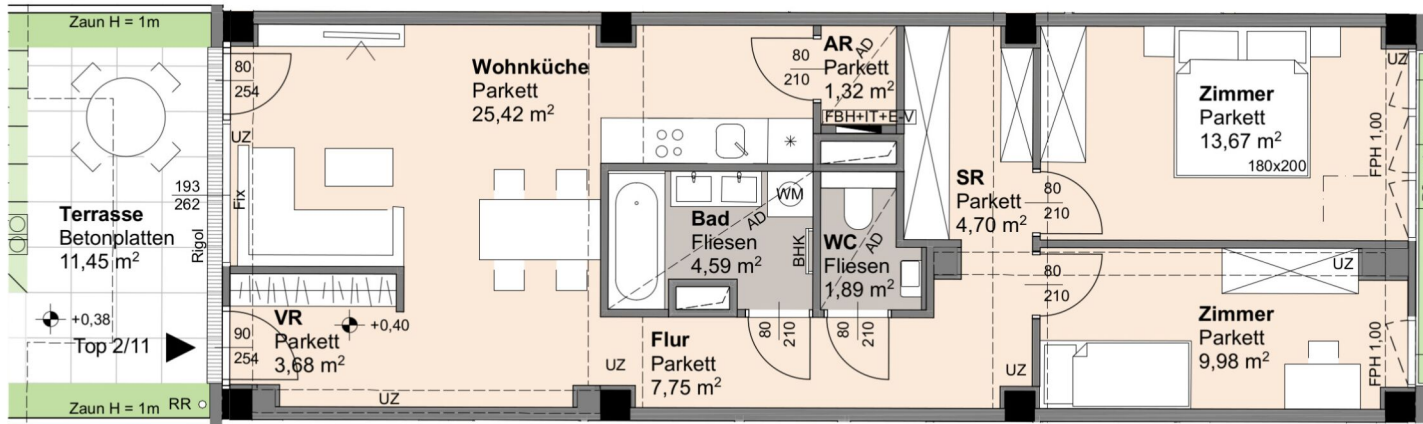
M = 1:100
