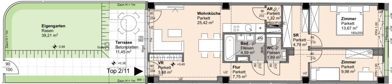
M = 1:150
